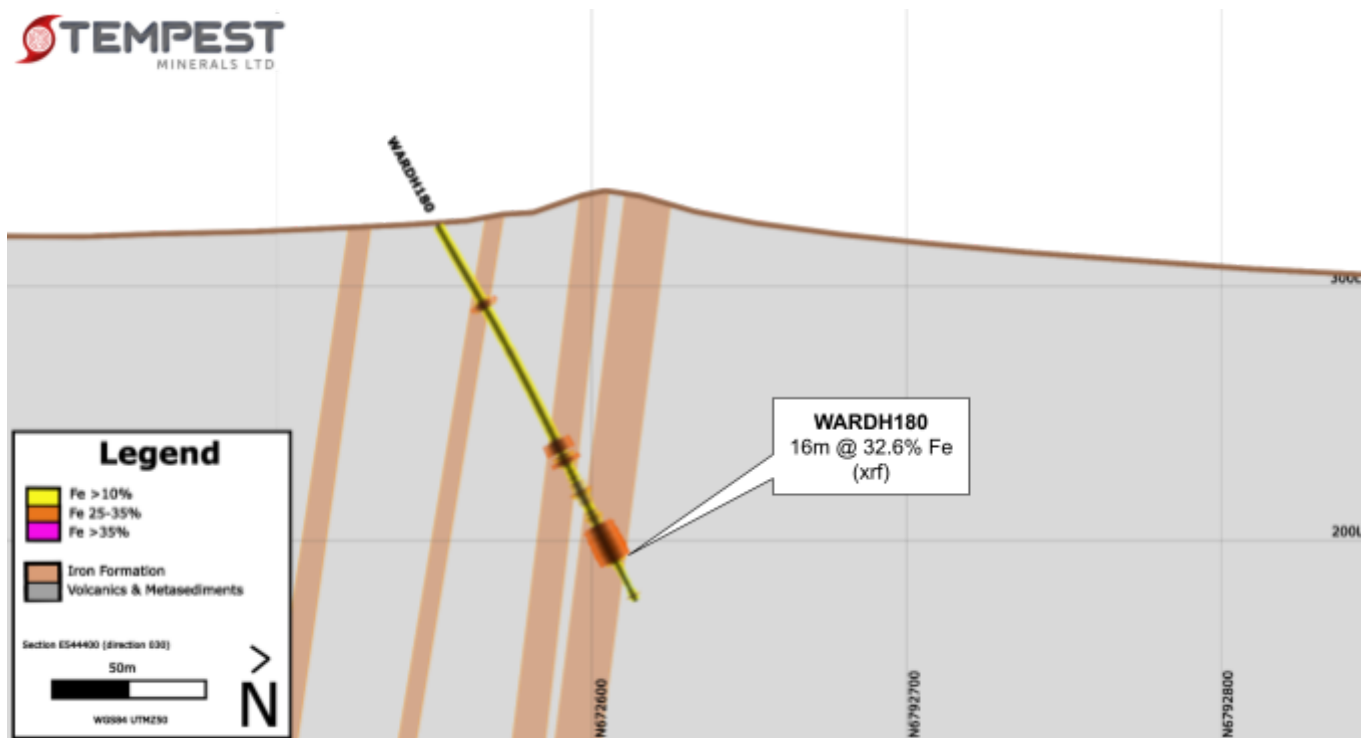
Figure 01: Section through iron mineralisation WARDH00180
