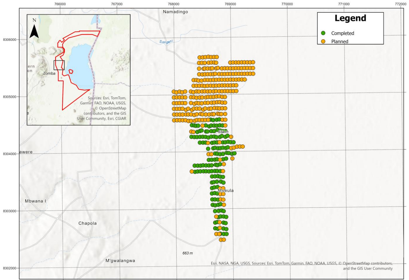
Figure 2: Drillhole locations at Bimbi showing the completed holes (results pending) and planned holes
