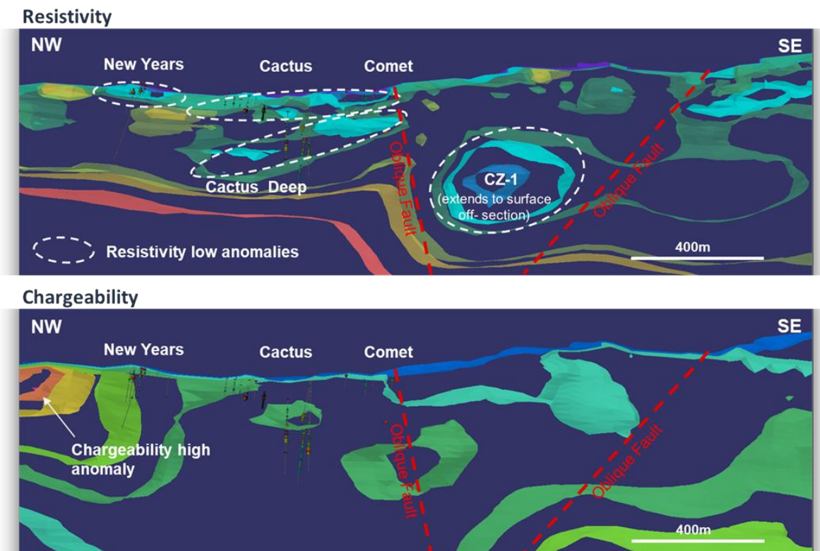
Figure 6: Resistivity and chargeability sections along the northwest-southeast IP section line shown in Figure 5. Cactus, Comet and New Years all have associated resistivity low anomalies. Additional key features include a very prominent resistivity low anomaly associated with the CZ-1 magnetic anomaly and a high order 50mV chargeability high coincident with the intrusive stock interpreted from magnetics.
