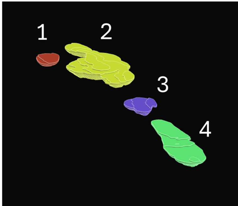
Figure 2: Horizon's Boorara Project initial pit optimisations
