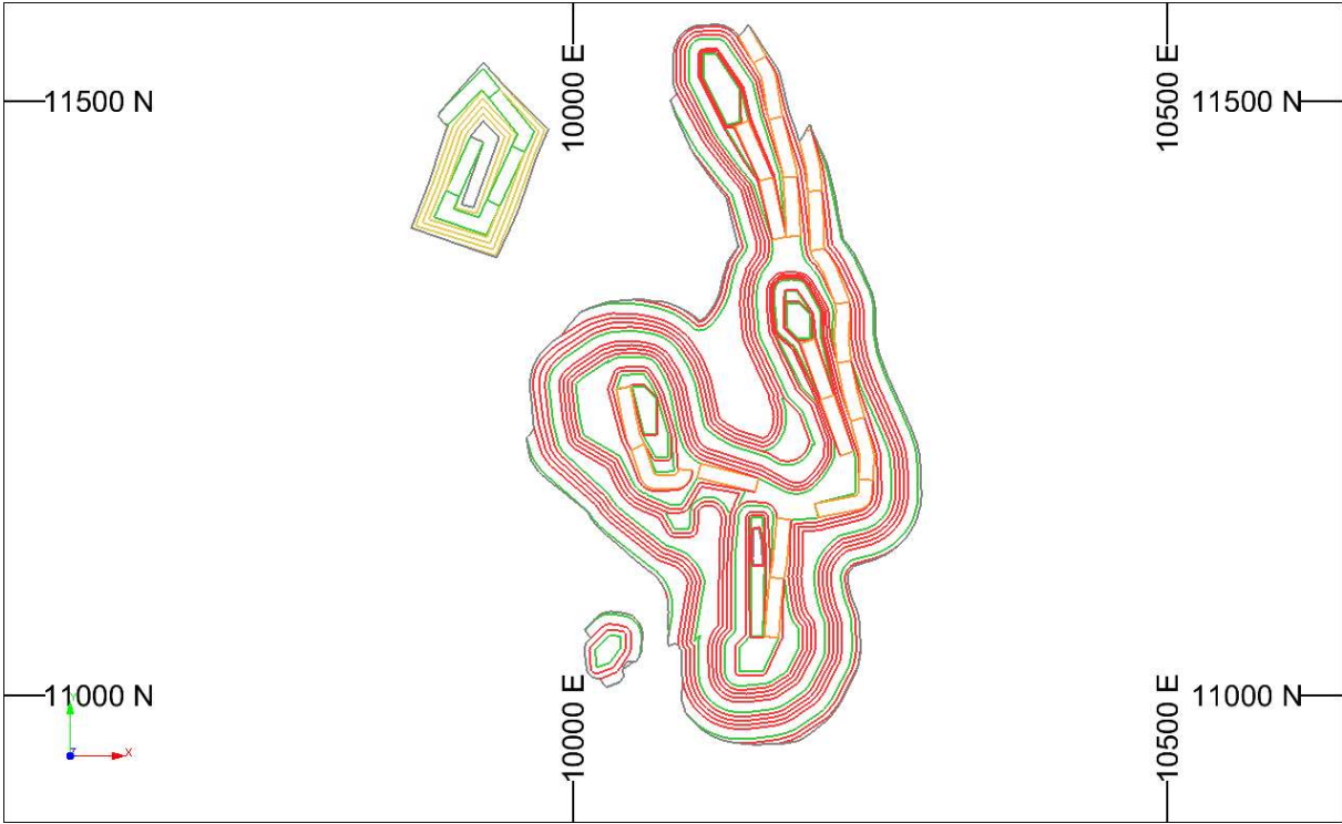
Figure 3: Pit design for Pit 1 and Pit 2
