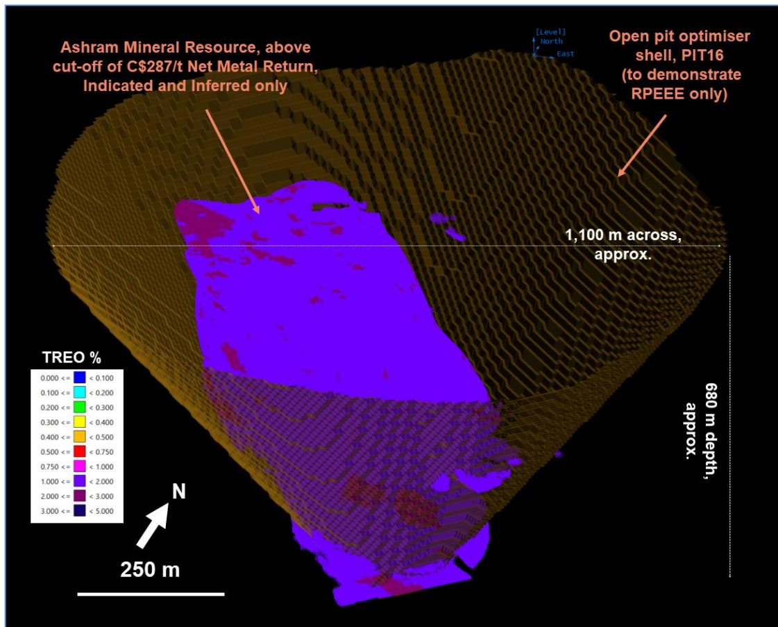
Figure 3.5.3 – Oblique view of Ashram Mineral Resource
