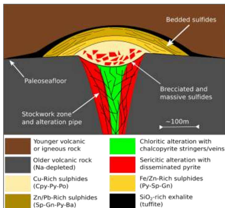
Figure 2.10: Typical volcanogenic massive sulfide cross section
