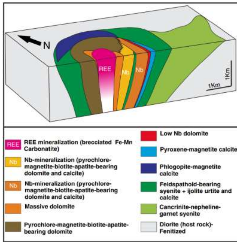
Figure 2.7: Schematic section of a carbonatite REE deposit
