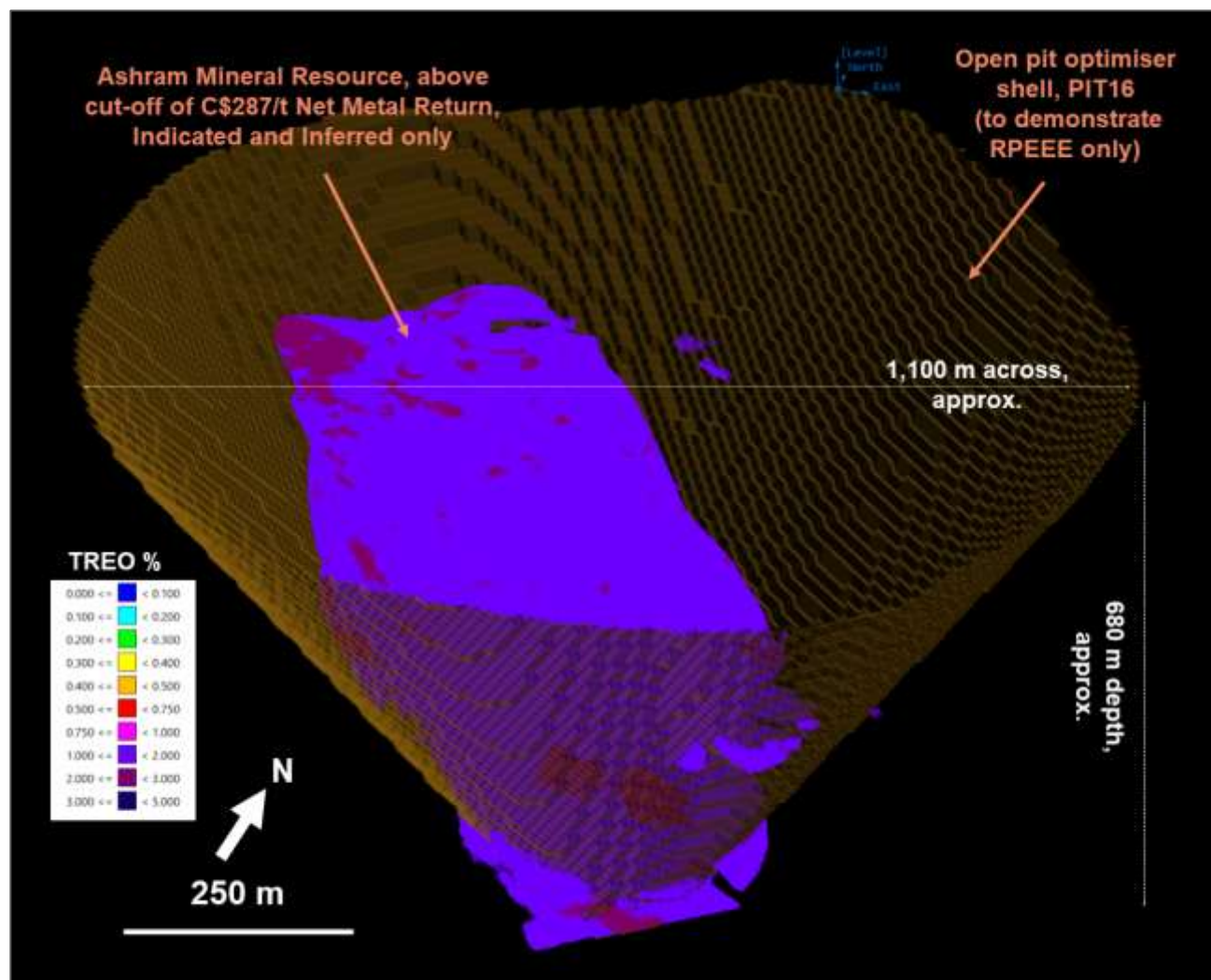
Figure 4.3: Oblique view of Ashram Mineral Resource
