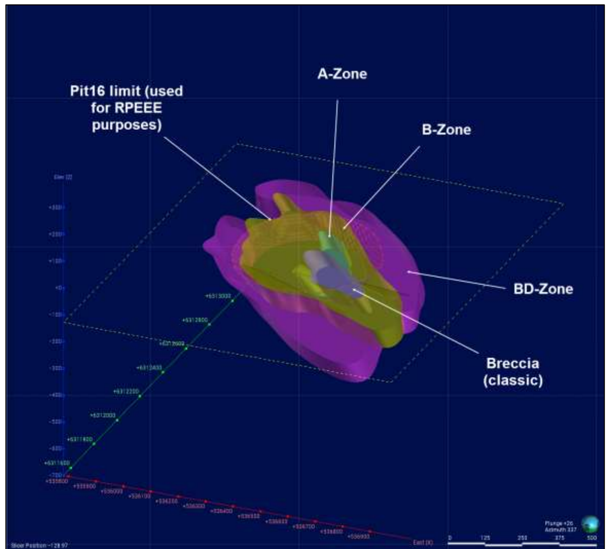
Figure 4.4: Mineralised domains at Ashram
