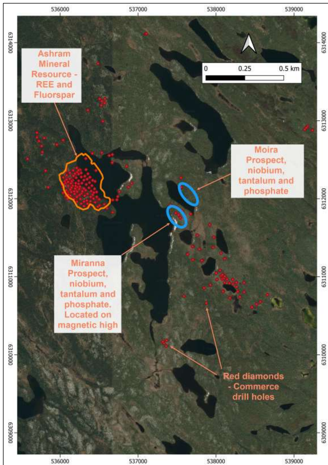
Figure 4.6: Exploration potential around the Ashram deposit, small scale
