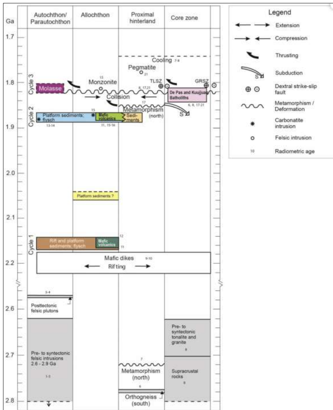
Figure 2.6: Tectonic history of New Quebec/Labrador Trough orogeny
