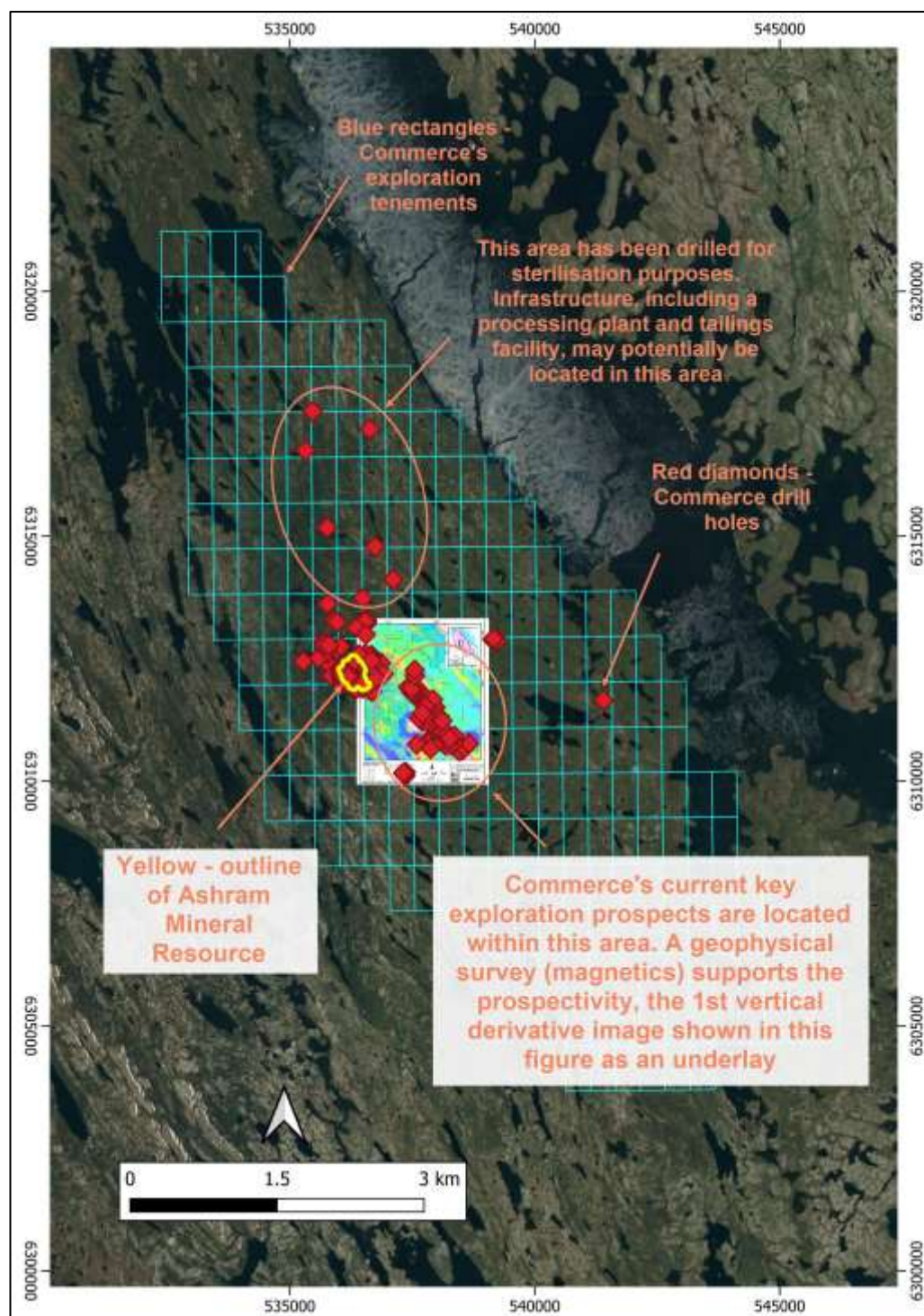
Figure 4.5: Exploration potential around the Ashram deposit, large scale
