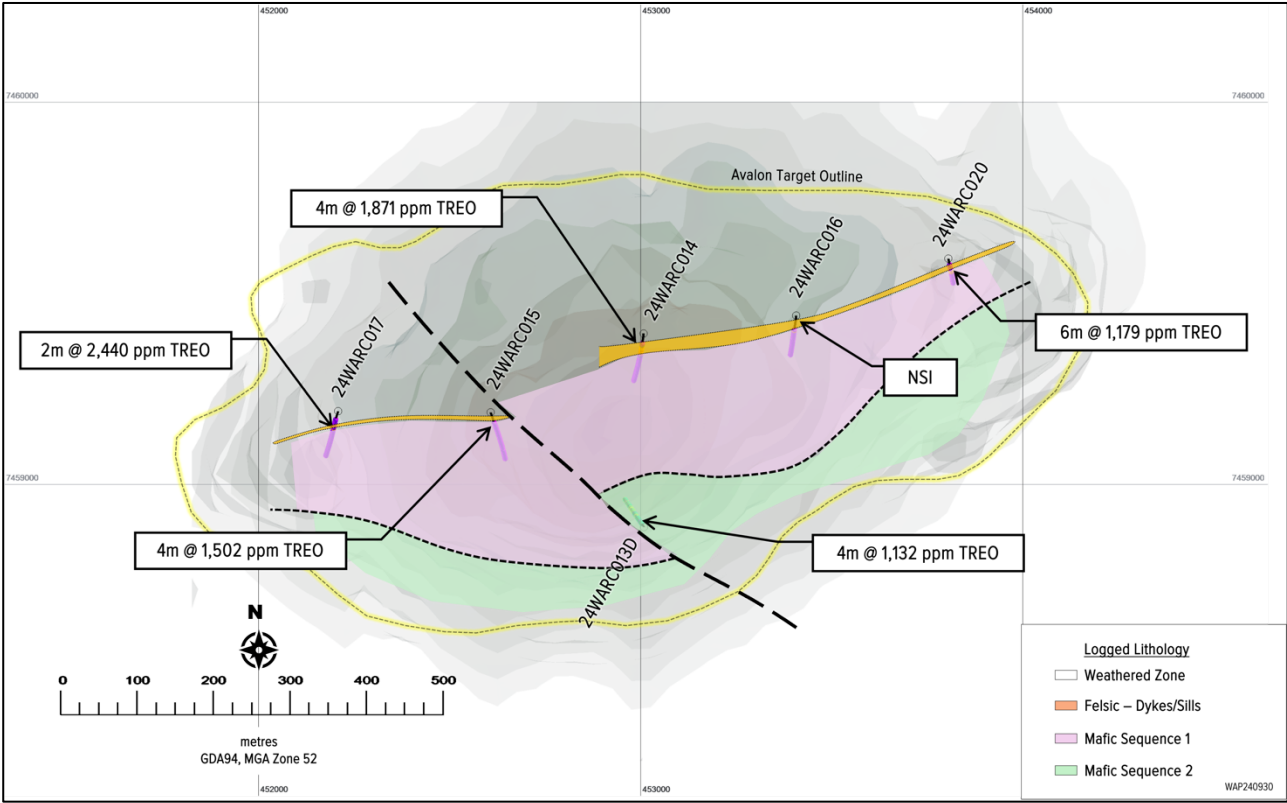
Figure 5 – Avalon drillhole location plan showing anomalous TREO intercepts, overlying a 3D-gravity density inversion model and geology interpretation.
